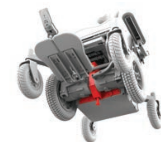
Figure 5.7d Frontier docking pin - extended
