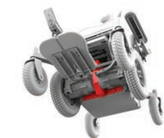
Figure 5.7c Frontier docking pin - retracted
