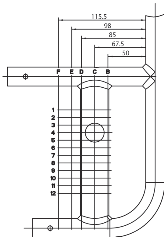
Drive wheel positions with CLT equipment
